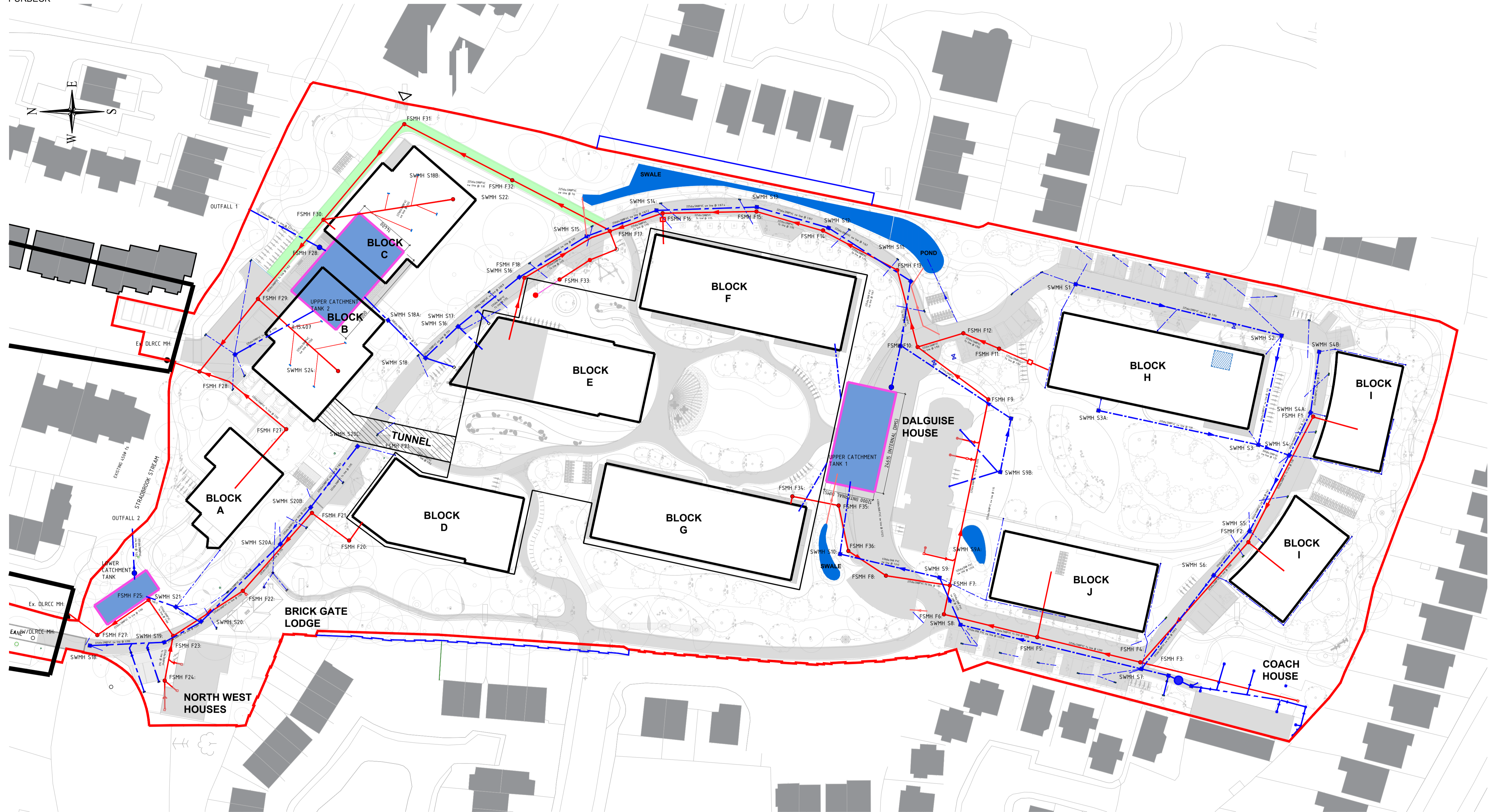
PROPOSED UTILITIES PLAN SCALE: 1:500
